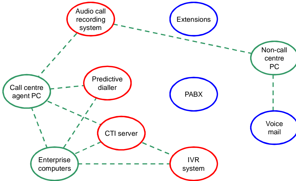
Figure 3 - Logical Architecture Illustrating Computing Links
